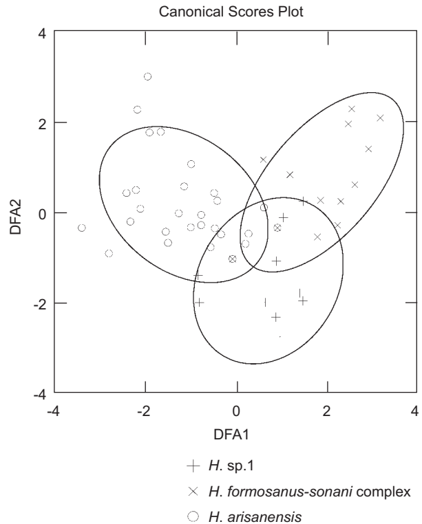
Fig. 3. Discriminant function analysis of the distributions of Hynobius arisanensis , the H. formosanus-sonani complex, and Hynobius sp. 1 in Taiwan. Canonical scores of the 3 groups with the 95% confidence interval of the means are plotted. Canonical scores of group means for the Alishan type are -1.13 for DFA1 and 0.20 for DFA2, for Nengao are 1.89 for DFA1 and 0.70 for DFA2, and for Nanhu are 0.72 for DFA1 and -1.48 for DFA2.
